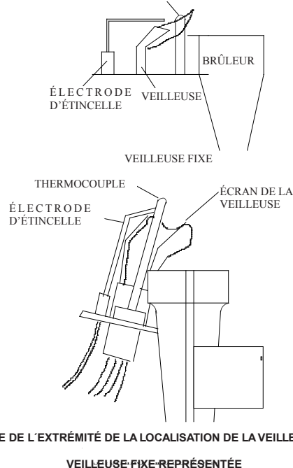
Figure 9 THERMOCOUPLE
